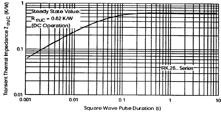
Fig. 11 - Thermal Impedance Z_{thJC} Characteristics
