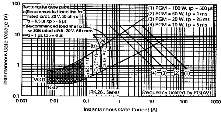
Fig. 12- Gate Characteristics
